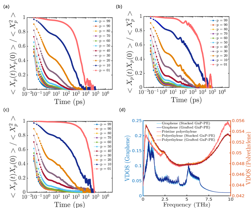
Figure 11. Rouse modes ( p = 99, 90, 80, 70, 60, 50, 40, 30, 20, 10 , and 01 ) for the (a) pristine PE, (b) stacked GnP–PE nanocomposite, and (c) grafted GnP–PE nanocomposite at T = 300 K. The autocorrelation function is normalized to scale the characteristic time scale. (d) Comparison of the partial VDOS of Gr and PE for the nanocomposites.
